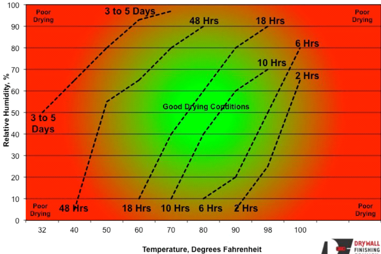
Joint Compound Drying Time As a function of temperature at specific relative humidity
